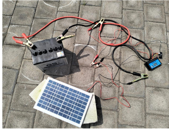
4.2 Rangkaian Panel Surya
