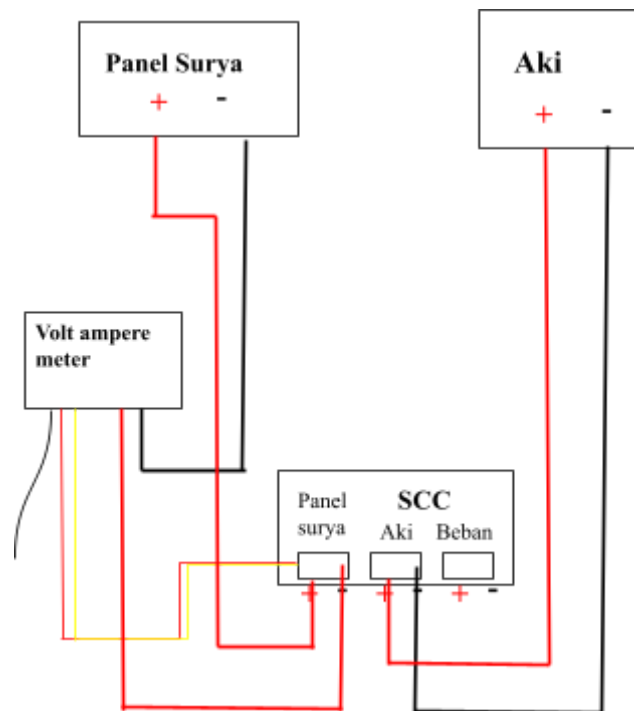
4.1 Diagram Rangkaian Panel Surya
